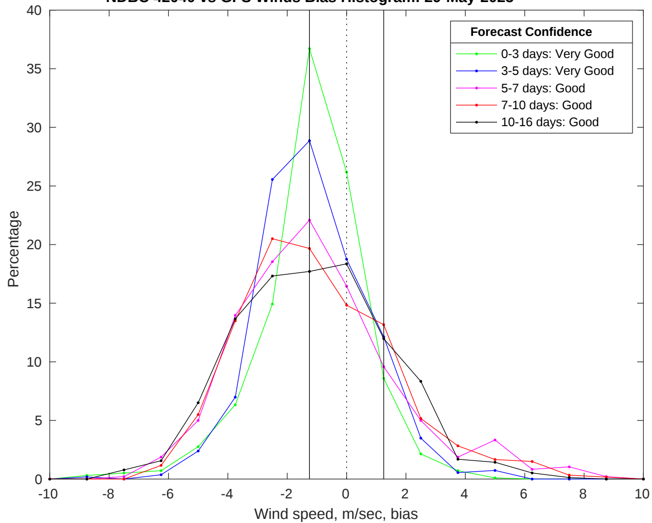
NDBC 42040 vs GFS Winds Bias Histogram: 29-May-2025
