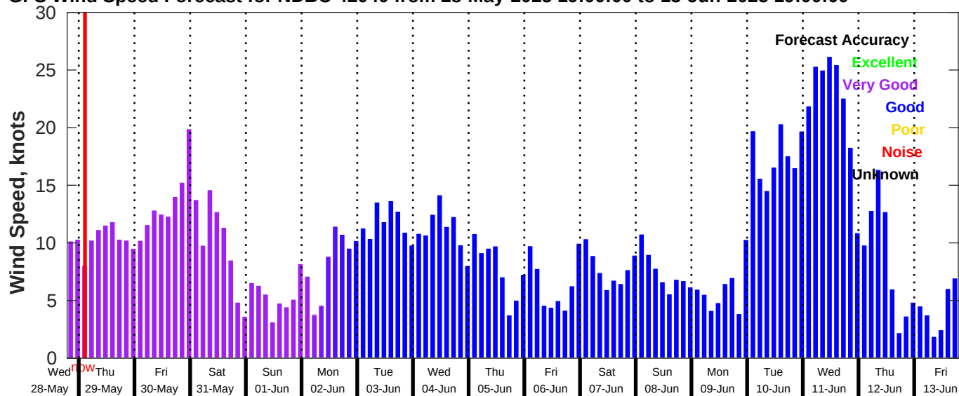
GFS Wind Speed Forecast for NDBC 42040 from 28-May-2025 19:00:00 to 13-Jun-2025 19:00:00
