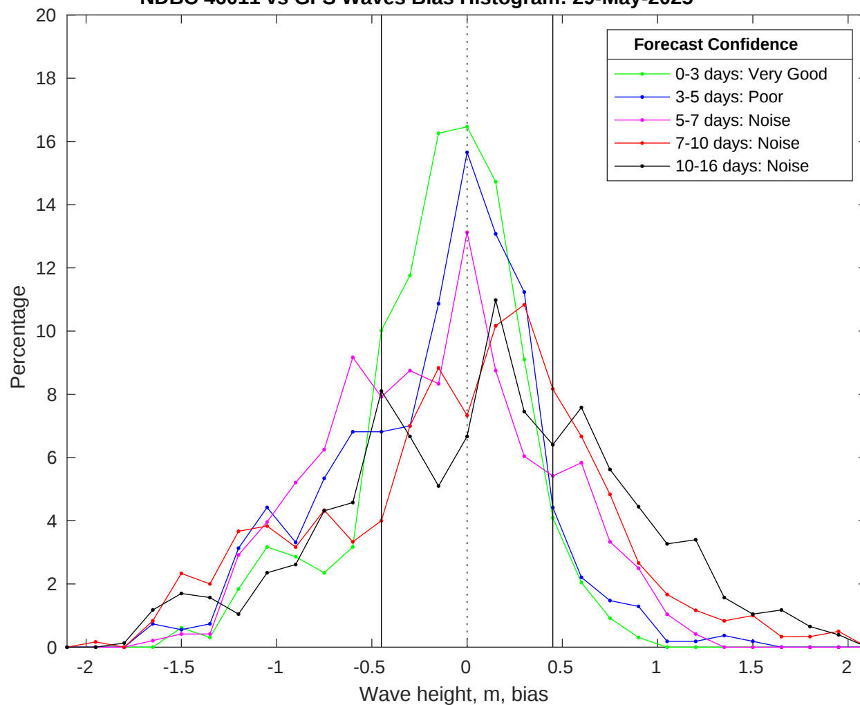
NDBC 46011 vs GFS Waves Bias Histogram: 29-May-2025
