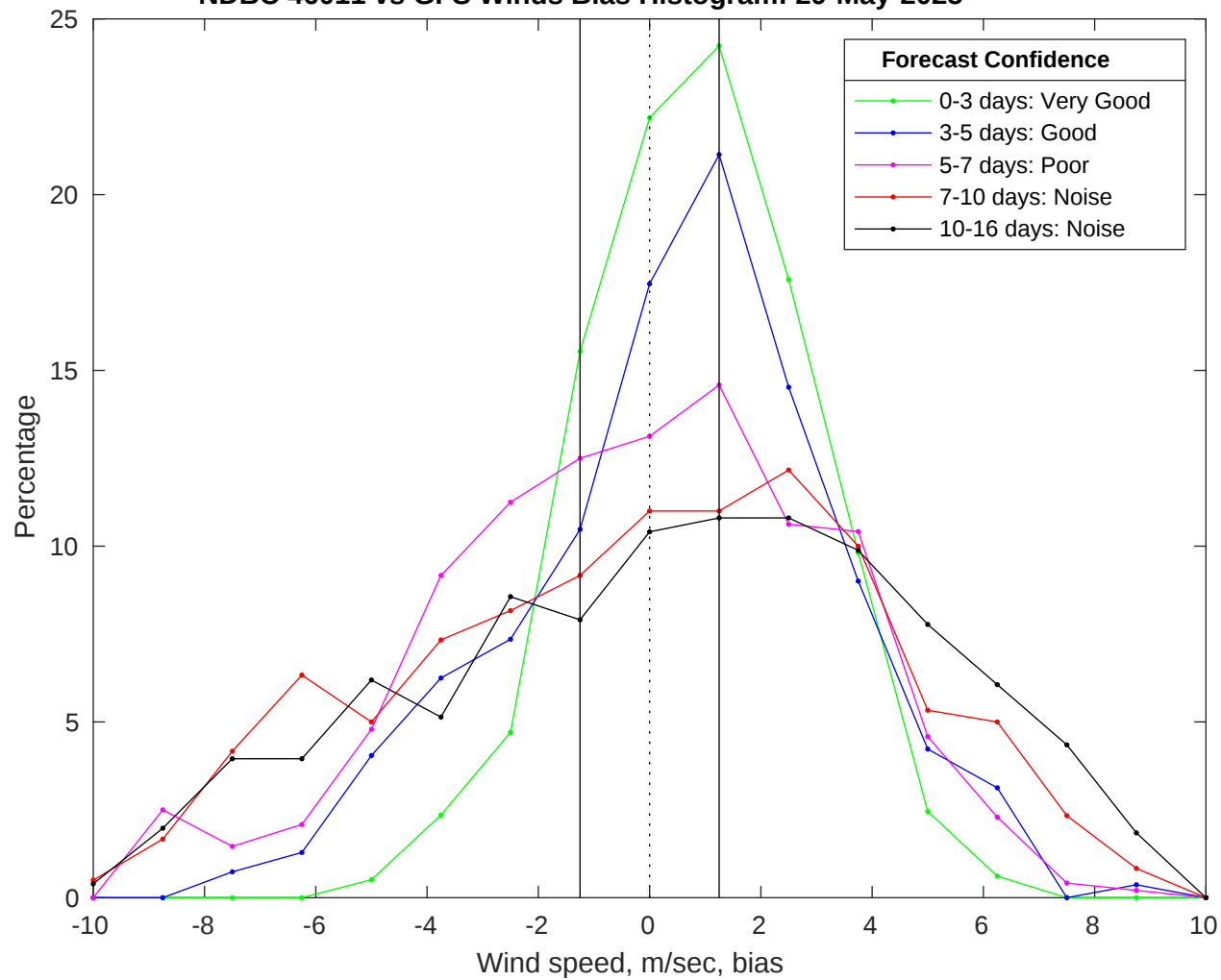
NDBC 46011 vs GFS Winds Bias Histogram: 29-May-2025
