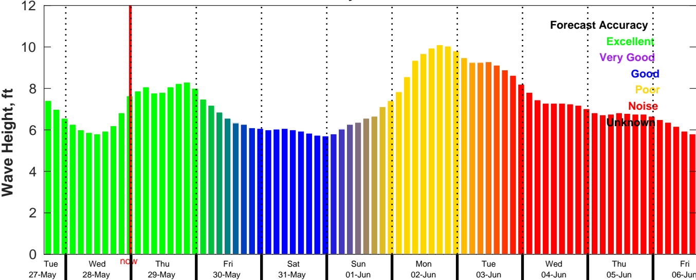
CMEMS Wave Forecast for NDBC 46011 from 27-May-2025 16:00:00 to 06-Jun-2025 16:00:00
