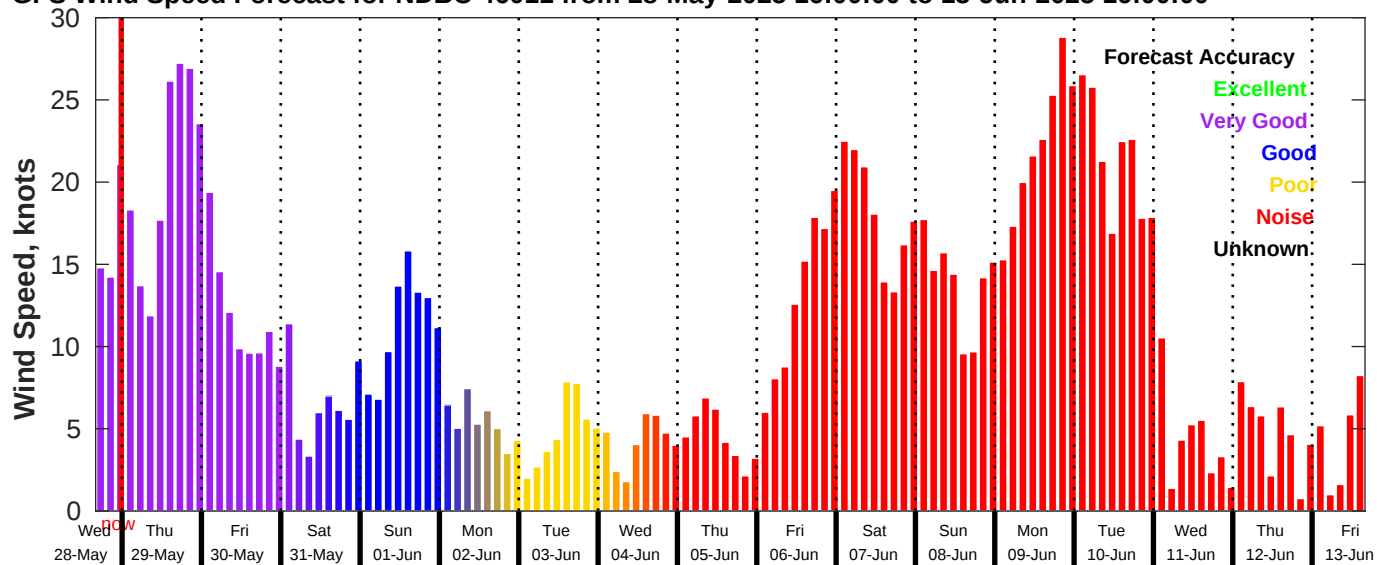
GFS Wind Speed Forecast for NDBC 46011 from 28-May-2025 16:00:00 to 13-Jun-2025 16:00:00
