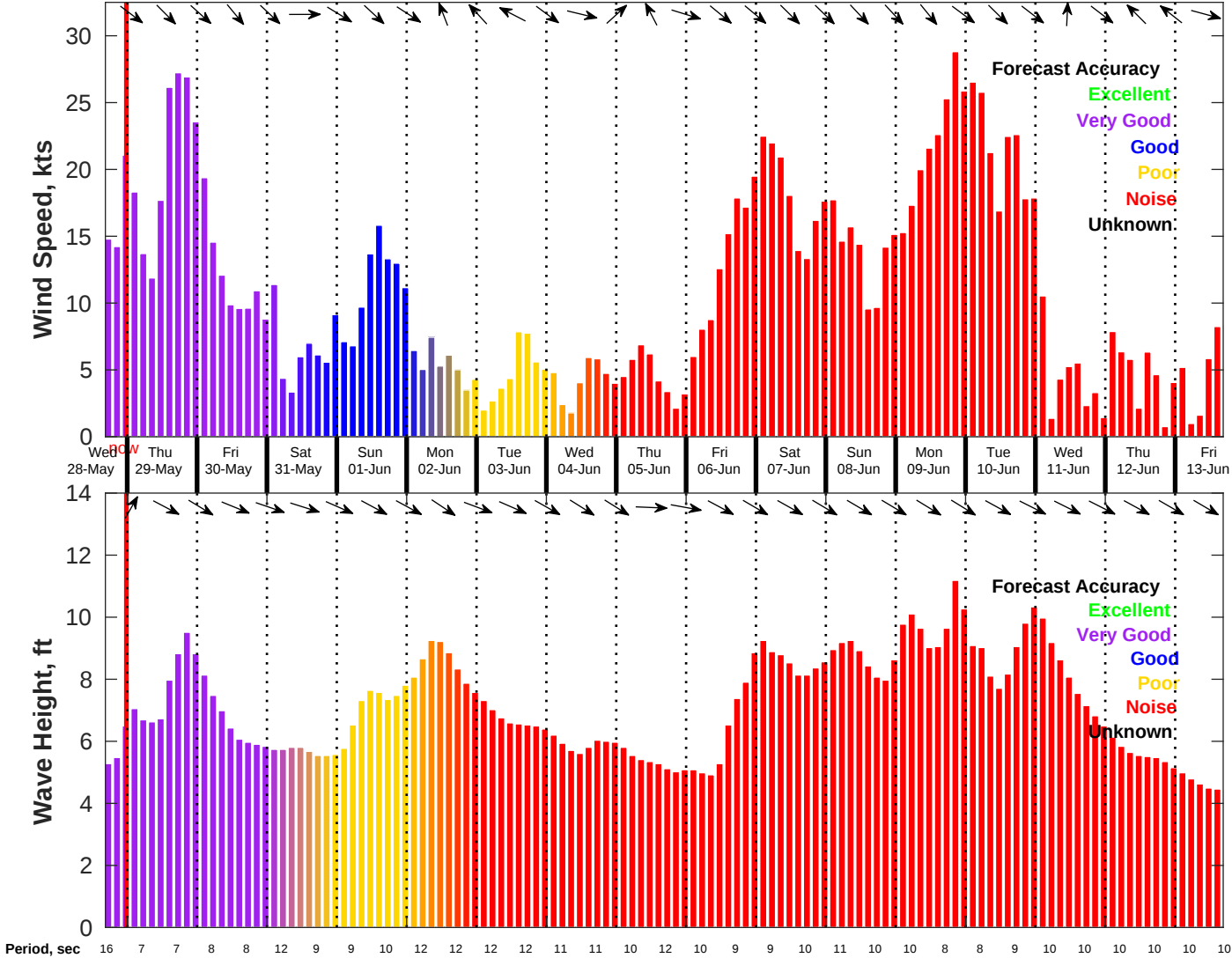
Wind & Wave Forecast for NDBC 46011 from 28-May-2025 16:00:00 to 13-Jun-2025 16:00:00
