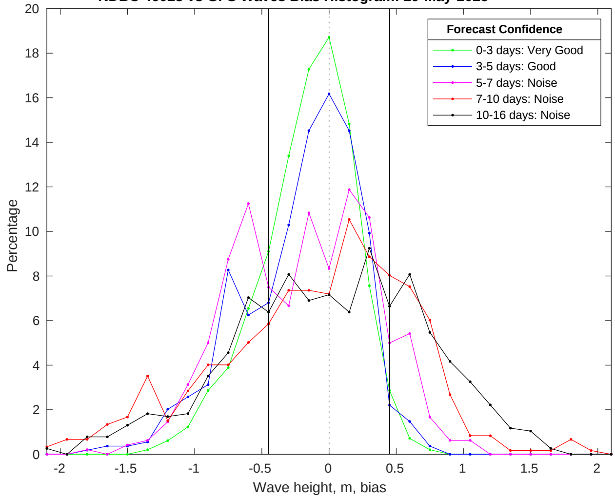
NDBC 46028 vs GFS Waves Bias Histogram: 29-May-2025
