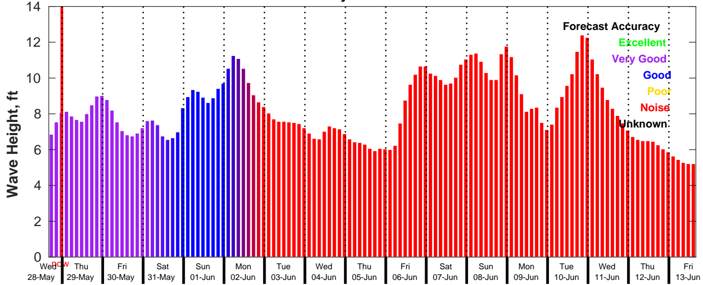
GFS Wave Forecast for NDBC 46028 from 28-May-2025 16:00:00 to 13-Jun-2025 16:00:00
