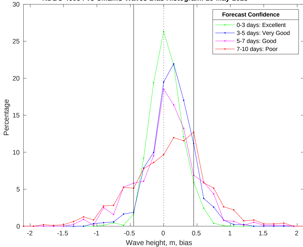
NDBC 46054 vs CMEMS Waves Bias Histogram: 29-May-2025
