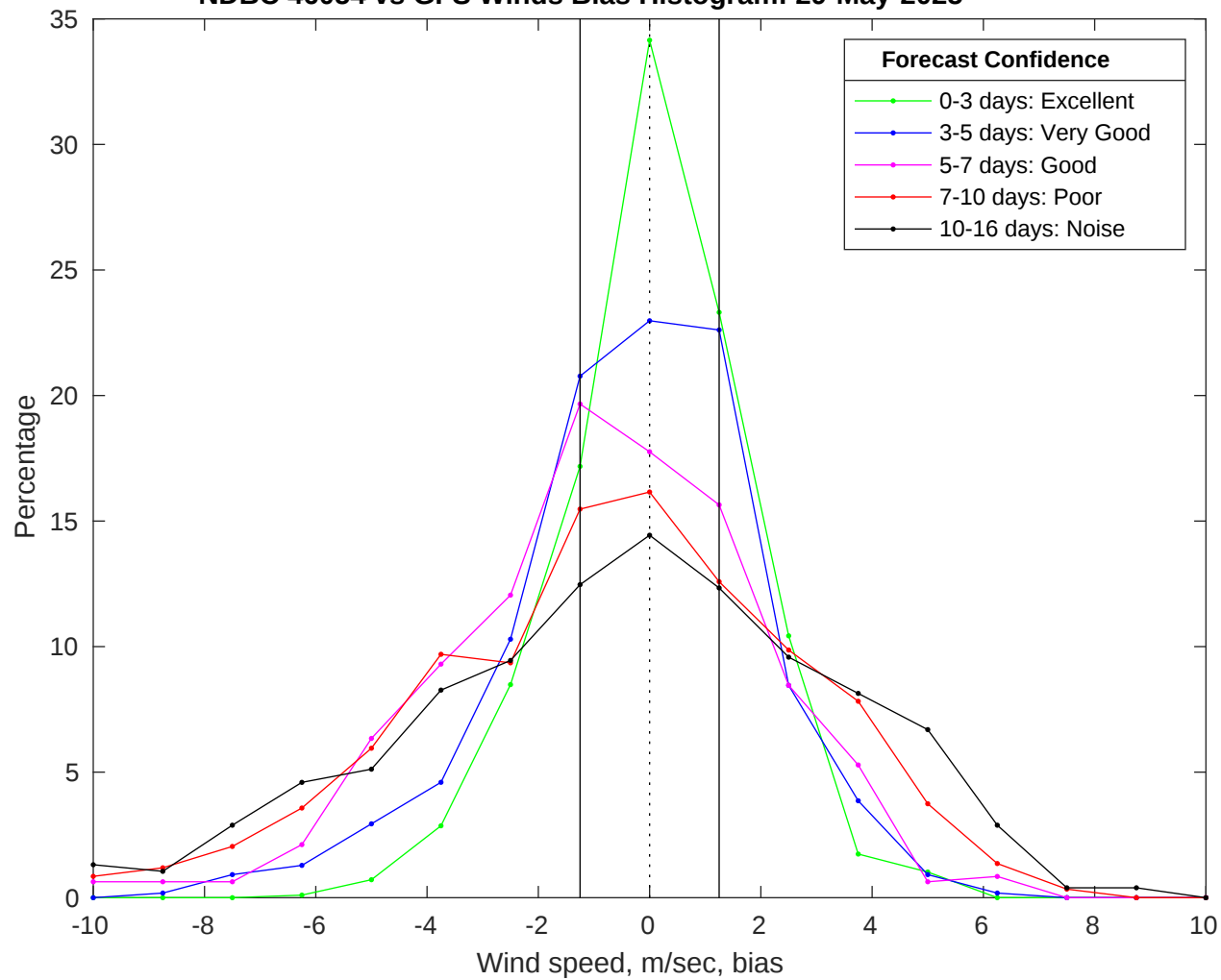
NDBC 46054 vs GFS Winds Bias Histogram: 29-May-2025
