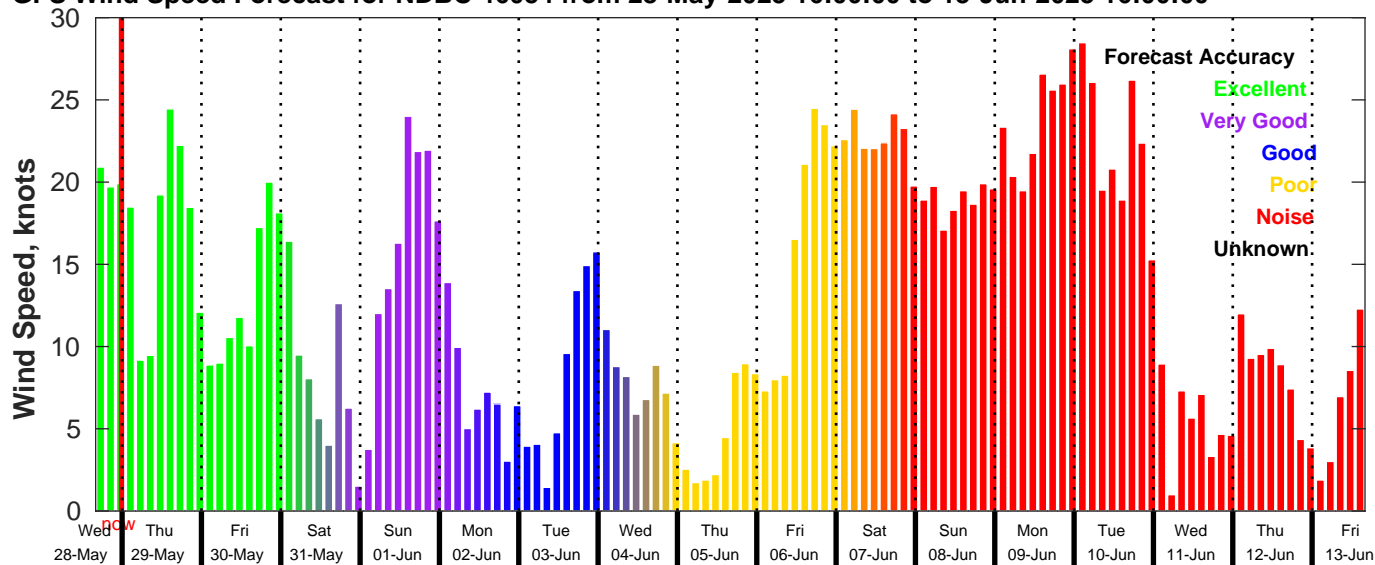
GFS Wind Speed Forecast for NDBC 46054 from 28-May-2025 16:00:00 to 13-Jun-2025 16:00:00
