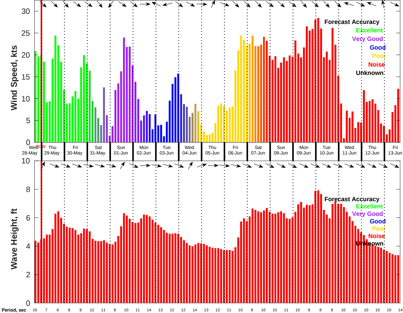
Wind & Wave Forecast for NDBC 46054 from 28-May-2025 16:00:00 to 13-Jun-2025 16:00:00
