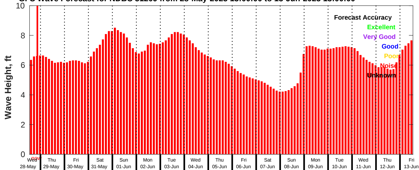
GFS Wave Forecast for NDBC 51209 from 28-May-2025 13:00:00 to 13-Jun-2025 13:00:00
