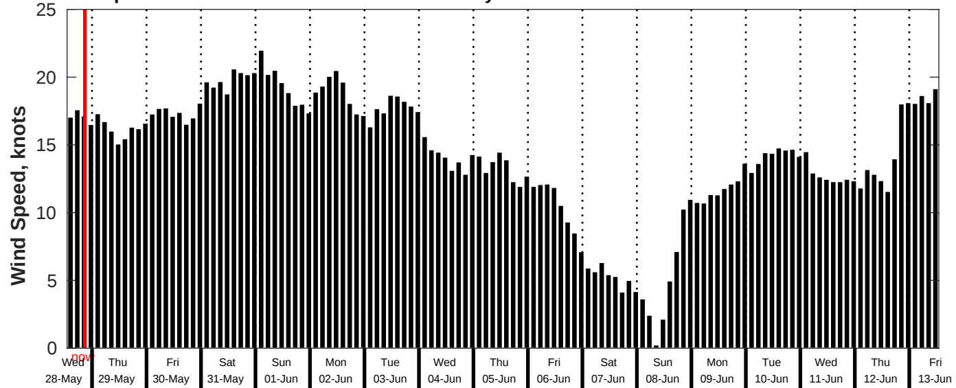
GFS Wind Speed Forecast for NDBC 51209 from 28-May-2025 13:00:00 to 13-Jun-2025 13:00:00
