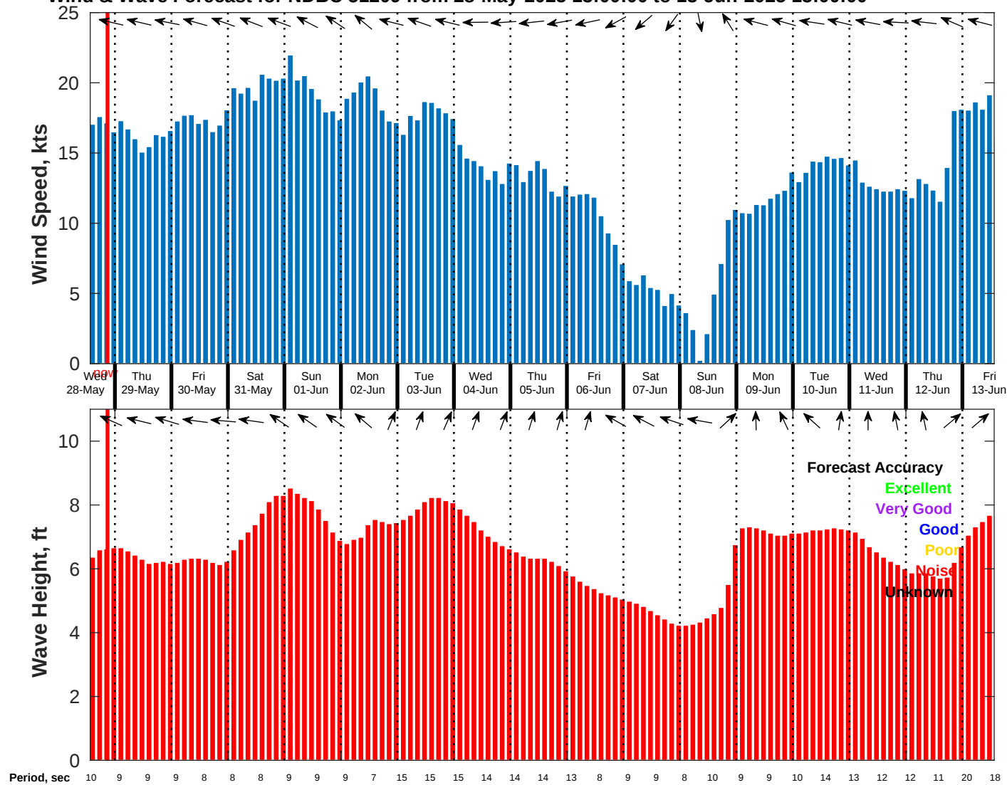
Wind & Wave Forecast for NDBC 51209 from 28-May-2025 13:00:00 to 13-Jun-2025 13:00:00
