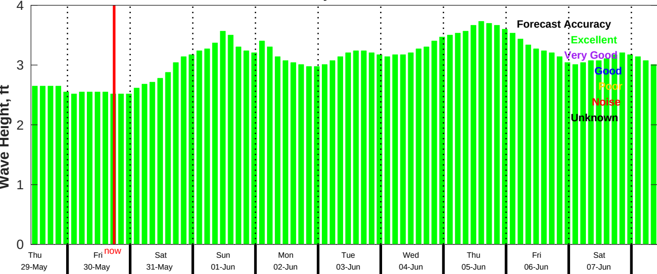
CMEMS Wave Forecast for NDBC 52211 from 28-May-2025 10:00:00 to 07-Jun-2025 10:00:00
