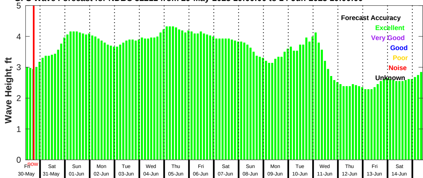
GFS Wave Forecast for NDBC 52211 from 29-May-2025 10:00:00 to 14-Jun-2025 10:00:00
