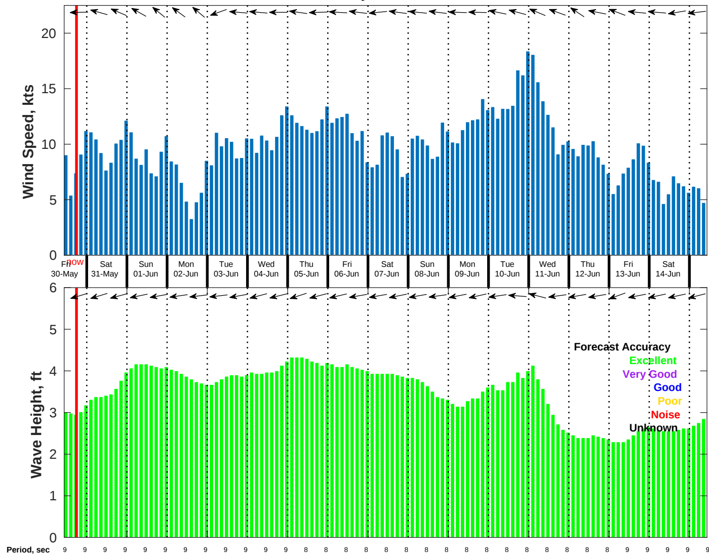
Wind & Wave Forecast for NDBC 52211 from 29-May-2025 10:00:00 to 14-Jun-2025 10:00:00
