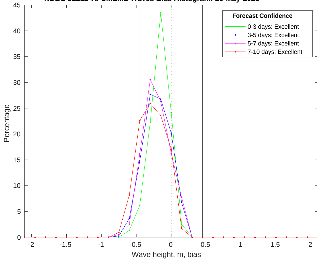
NDBC 52212 vs CMEMS Waves Bias Histogram: 29-May-2025
