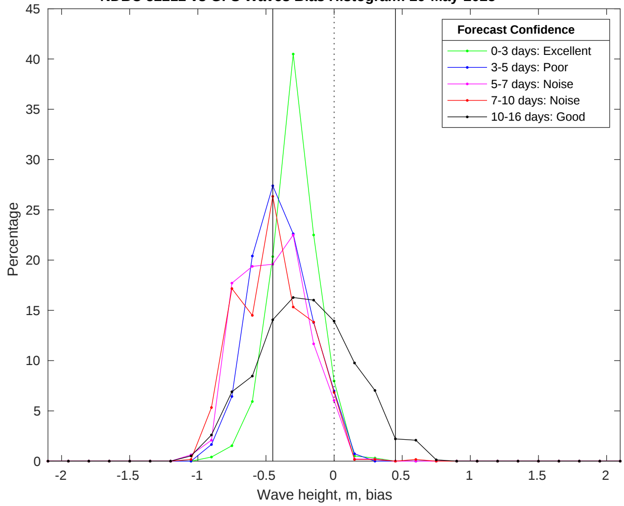
NDBC 52212 vs GFS Waves Bias Histogram: 29-May-2025
