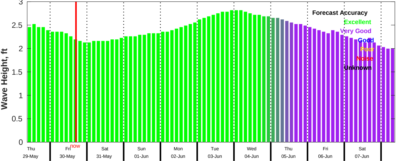
CMEMS Wave Forecast for NDBC 52212 from 28-May-2025 09:00:00 to 07-Jun-2025 09:00:00
