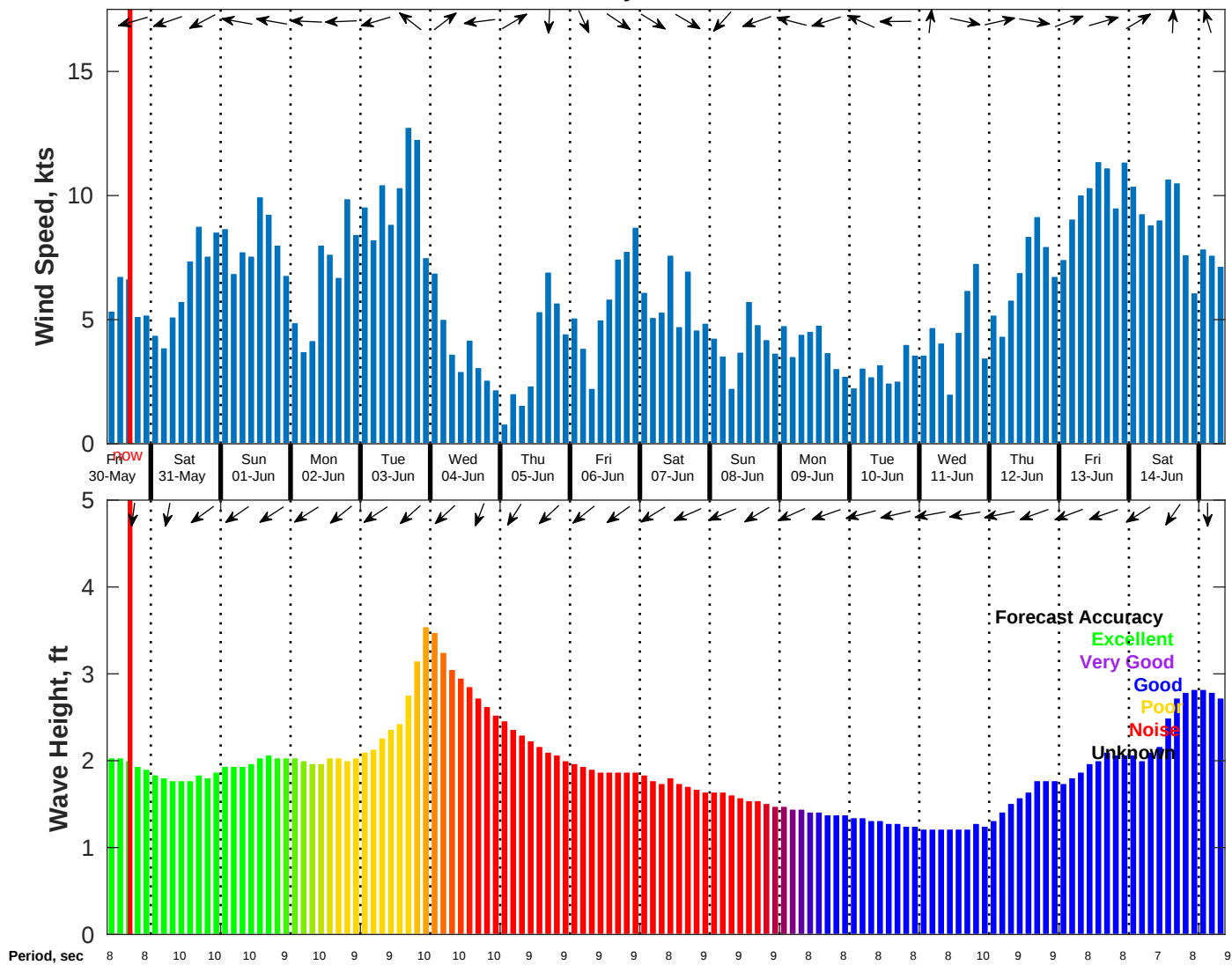
Wind & Wave Forecast for NDBC 52212 from 29-May-2025 09:00:00 to 14-Jun-2025 09:00:00
