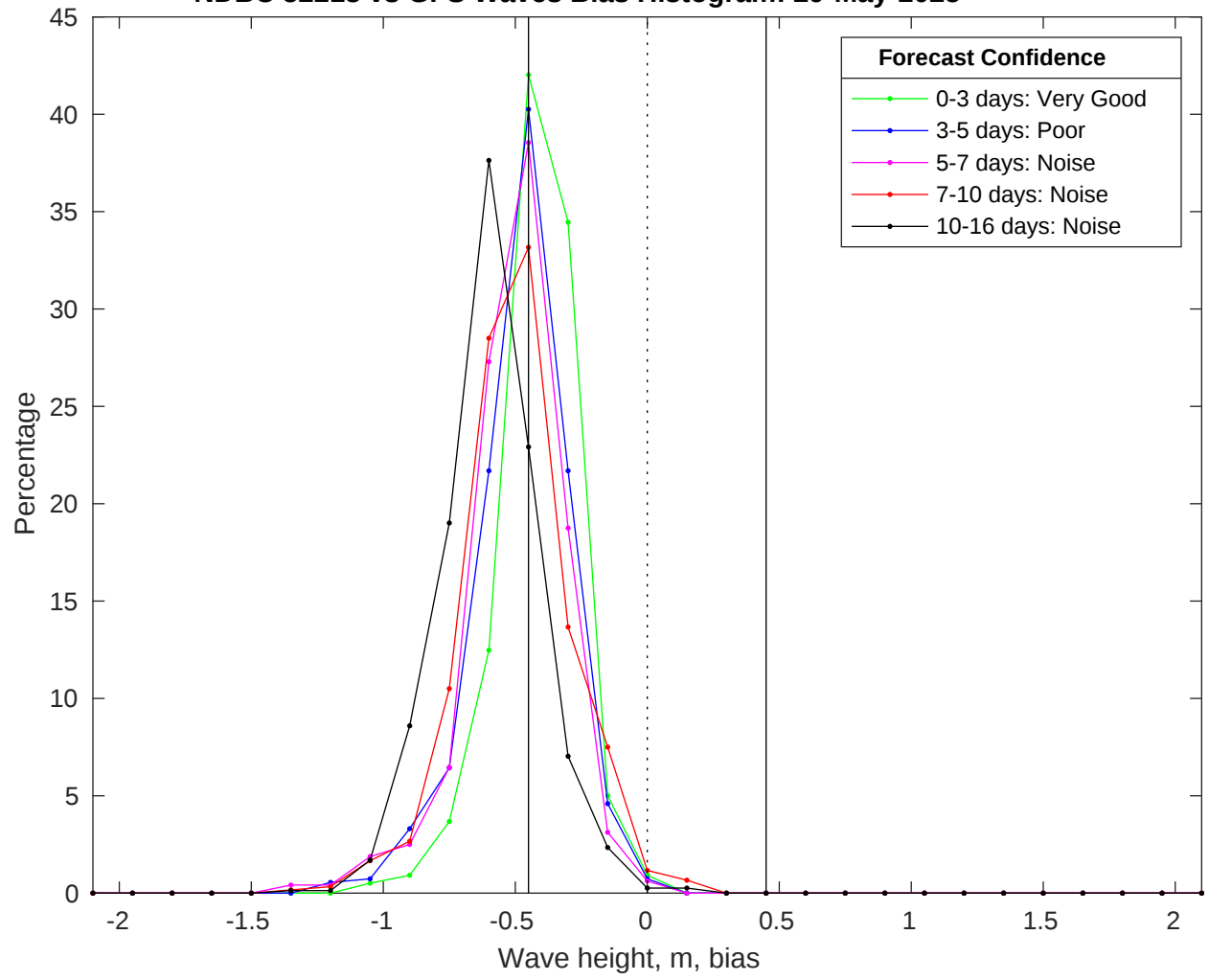
NDBC 52213 vs GFS Waves Bias Histogram: 29-May-2025
