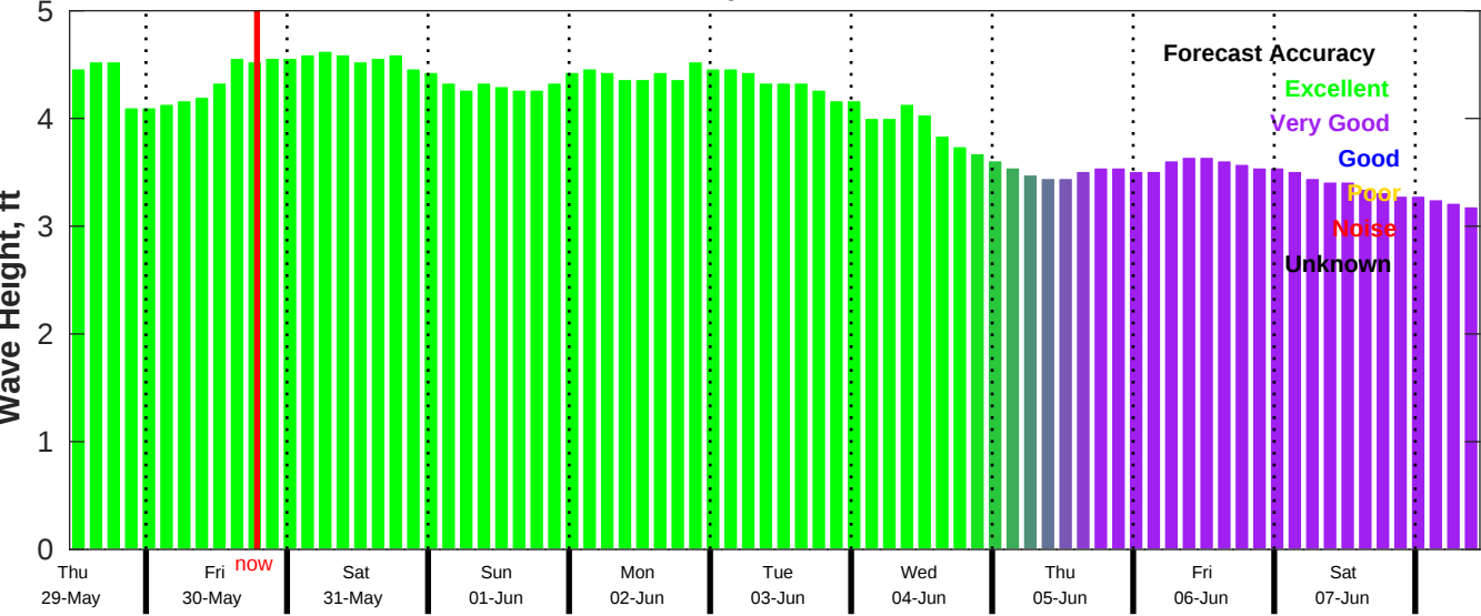
CMEMS Wave Forecast for NDBC 52213 from 28-May-2025 11:00:00 to 07-Jun-2025 11:00:00
