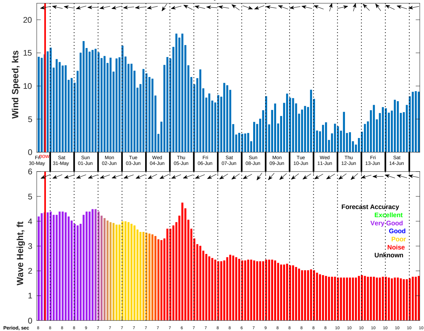
Wind & Wave Forecast for NDBC 52213 from 29-May-2025 11:00:00 to 14-Jun-2025 11:00:00
