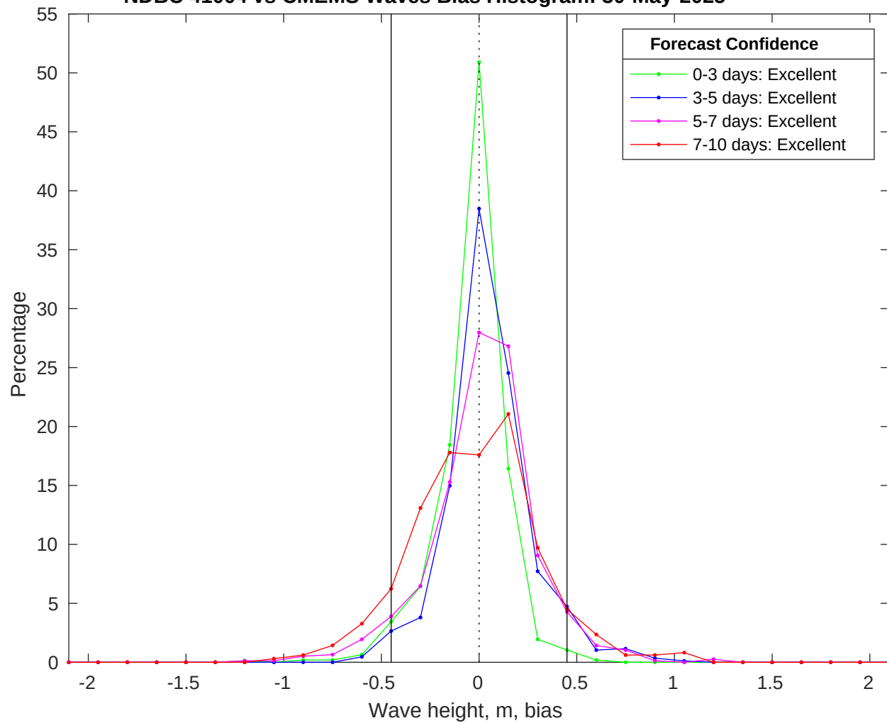
NDBC 41004 vs CMEMS Waves Bias Histogram: 30-May-2025
