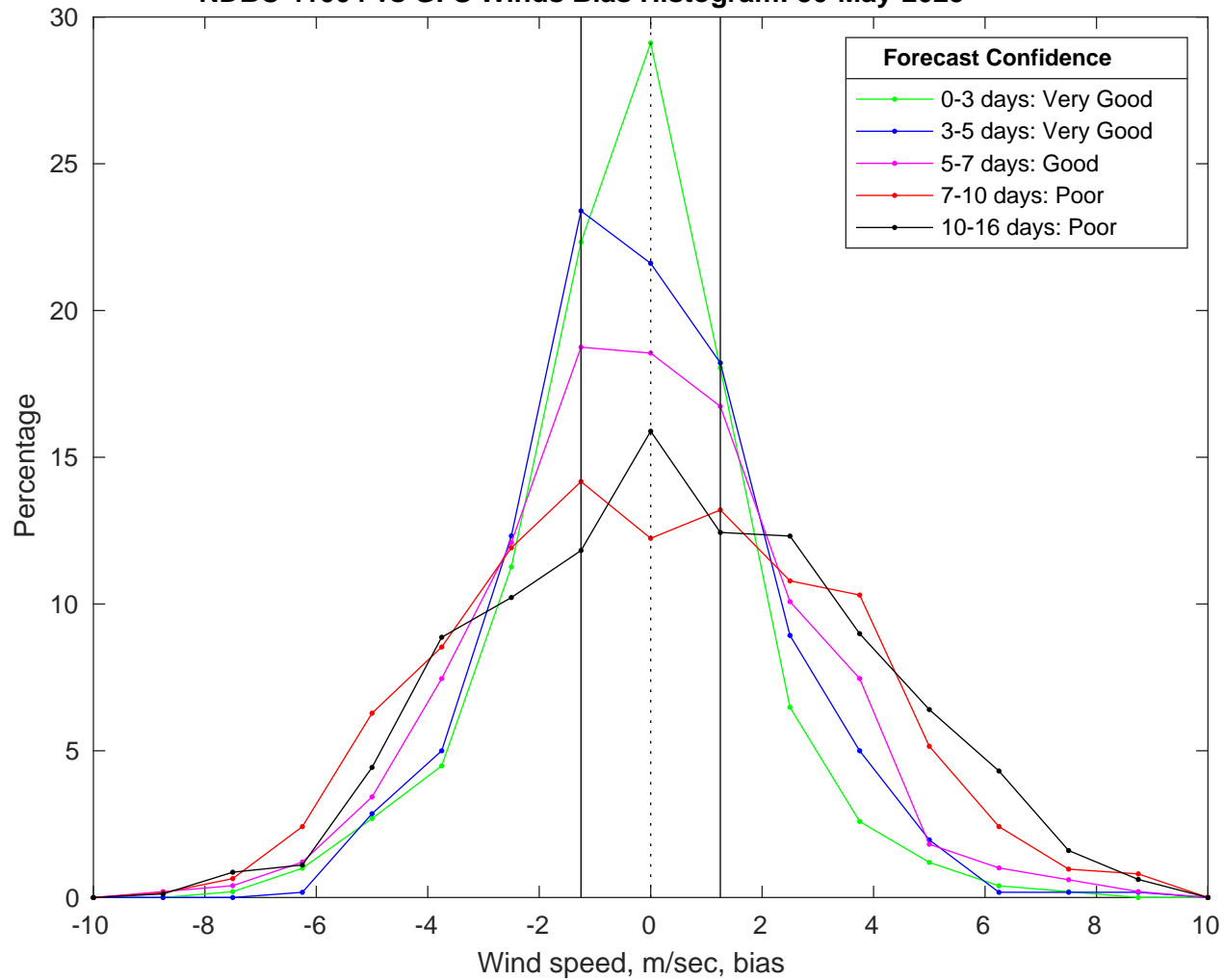
NDBC 41004 vs GFS Winds Bias Histogram: 30-May-2025
