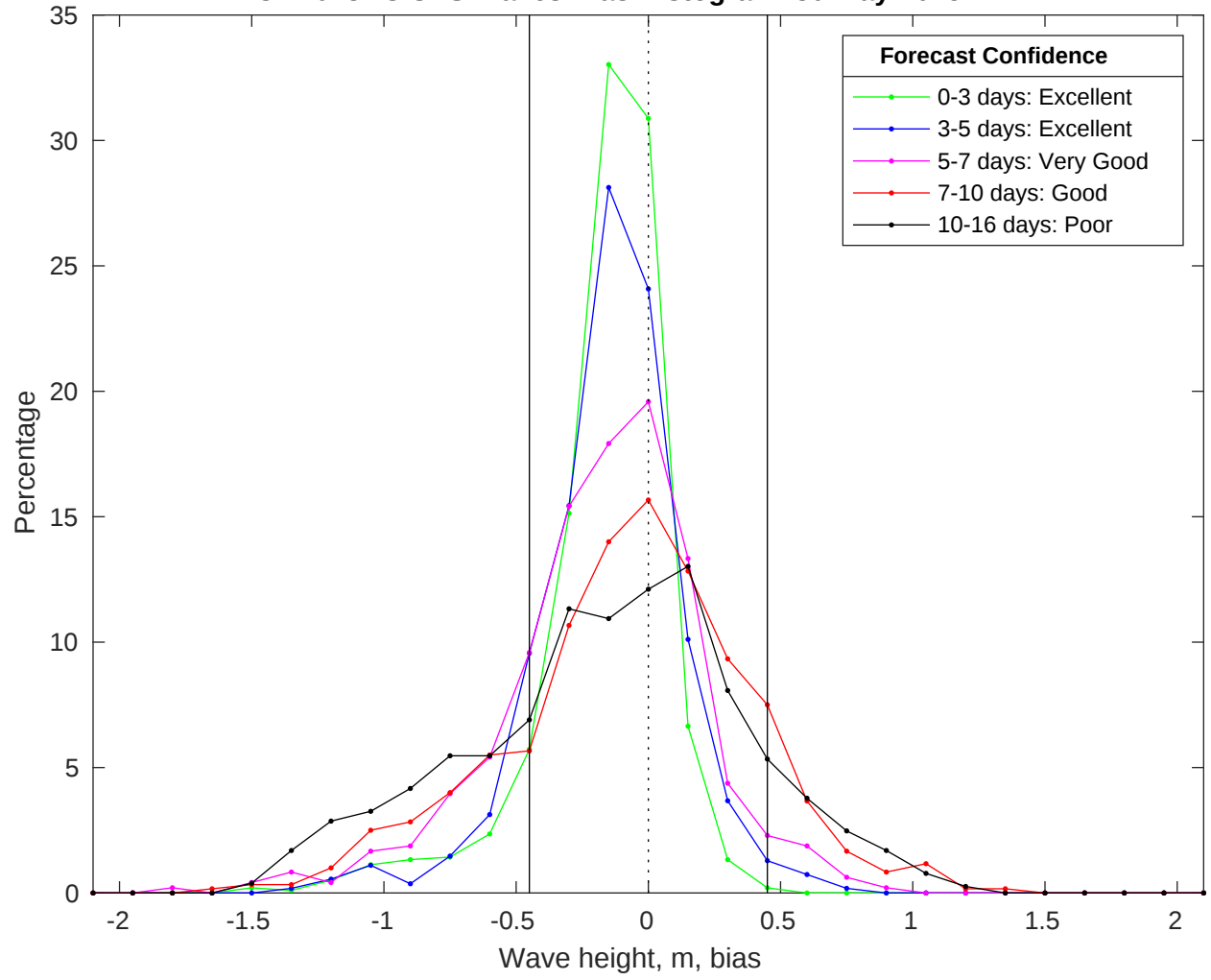
NDBC 41013 vs GFS Waves Bias Histogram: 30-May-2025
