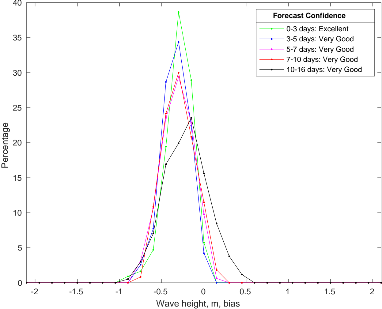
NDBC 41040 vs GFS Waves Bias Histogram: 30-May-2025
