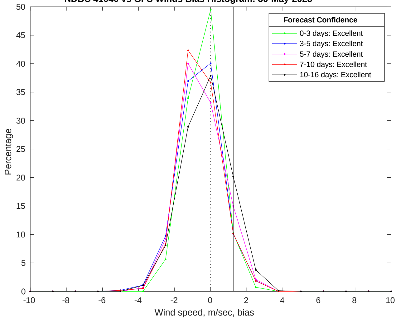
NDBC 41040 vs GFS Winds Bias Histogram: 30-May-2025
