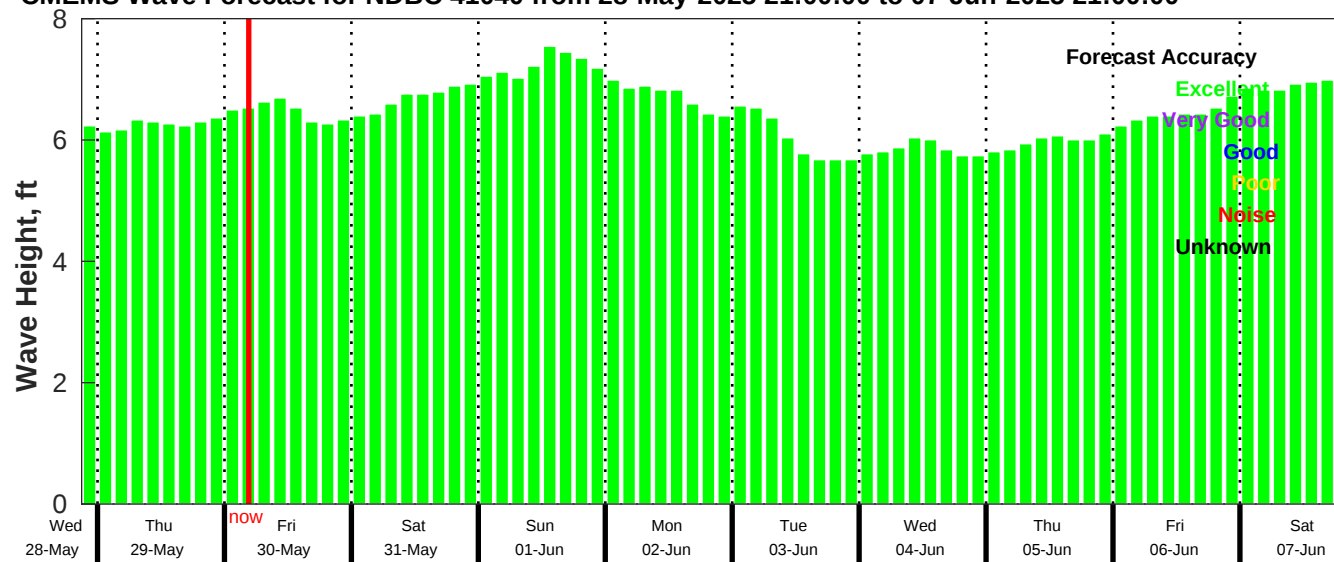
CMEMS Wave Forecast for NDBC 41040 from 28-May-2025 21:00:00 to 07-Jun-2025 21:00:00
