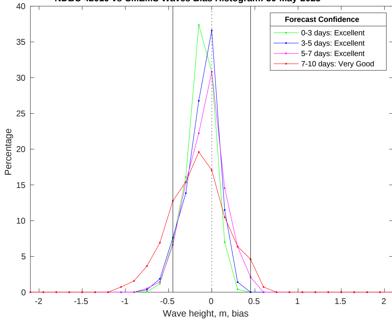
NDBC 42019 vs CMEMS Waves Bias Histogram: 30-May-2025
