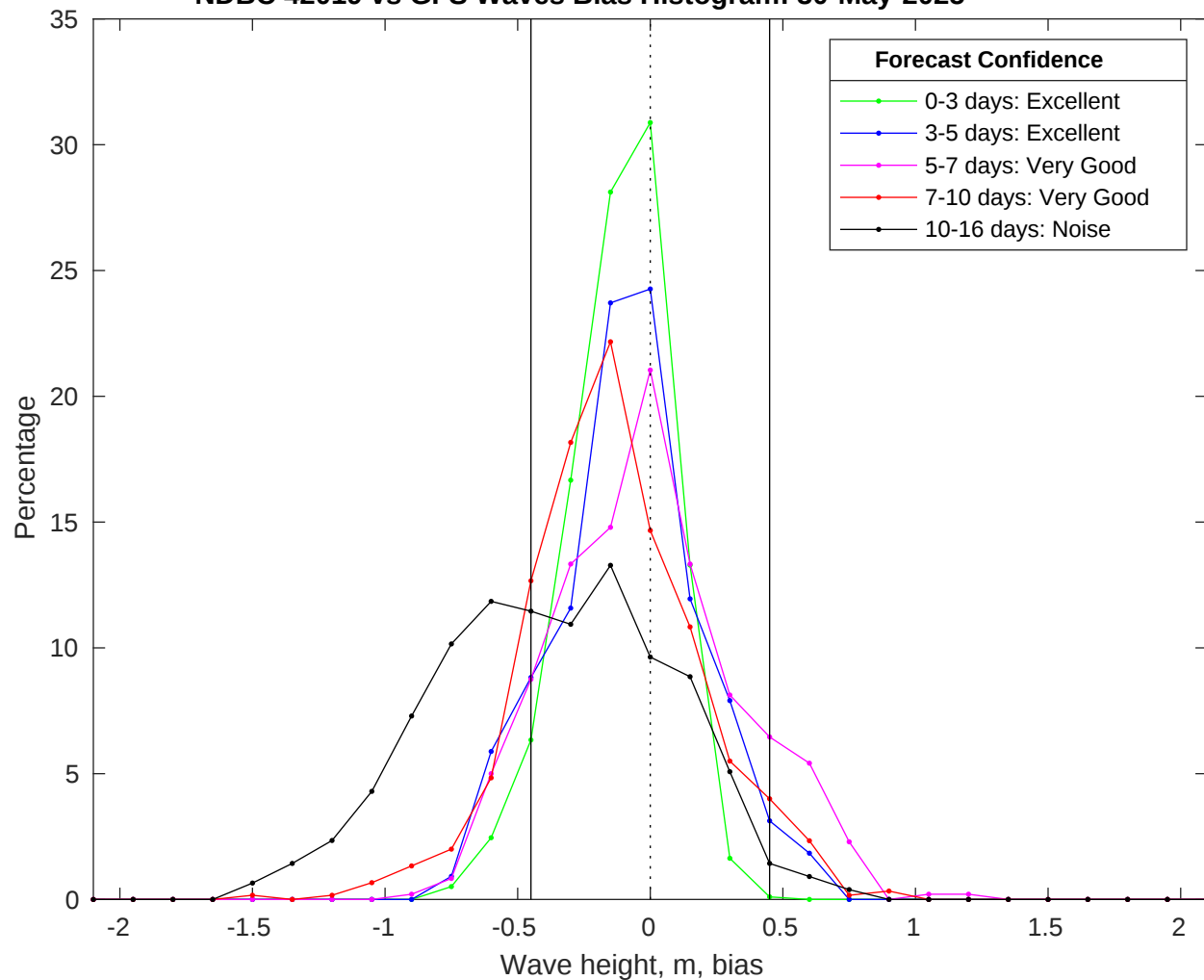
NDBC 42019 vs GFS Waves Bias Histogram: 30-May-2025
