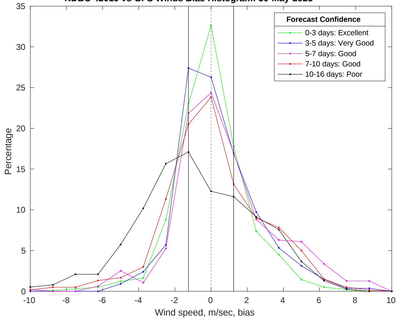
NDBC 42019 vs GFS Winds Bias Histogram: 30-May-2025
