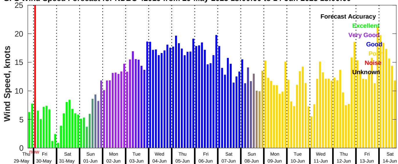
GFS Wind Speed Forecast for NDBC 42019 from 29-May-2025 18:00:00 to 14-Jun-2025 18:00:00
