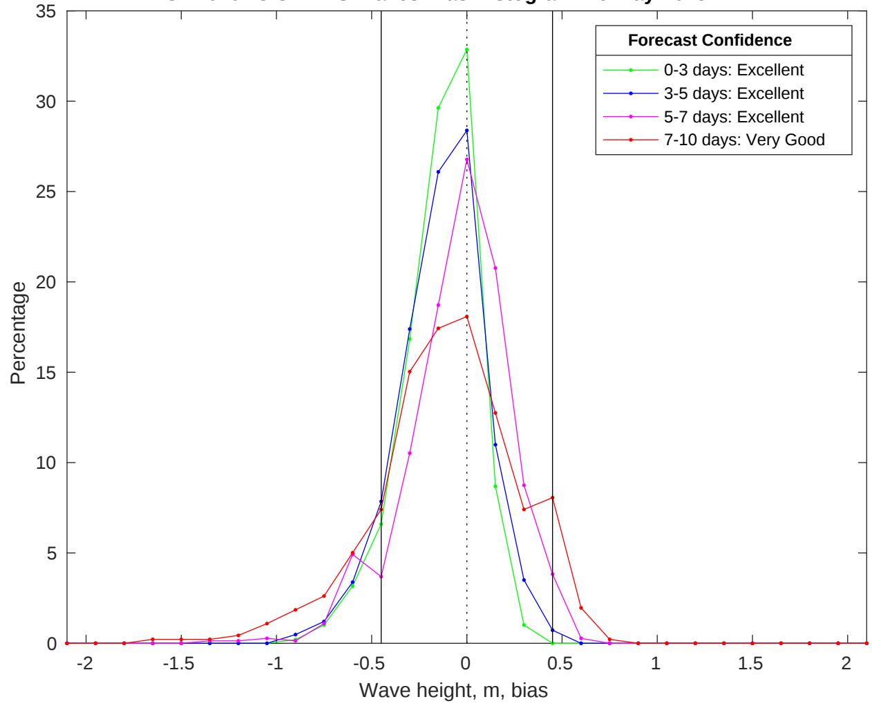
NDBC 42020 vs CMEMS Waves Bias Histogram: 29-May-2025
