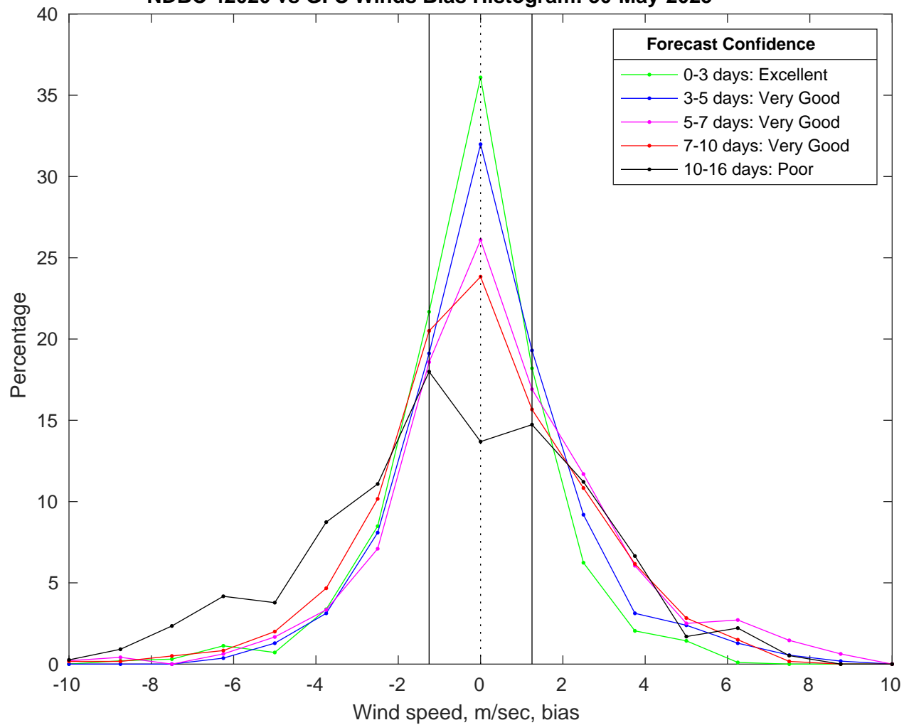
NDBC 42020 vs GFS Winds Bias Histogram: 30-May-2025
