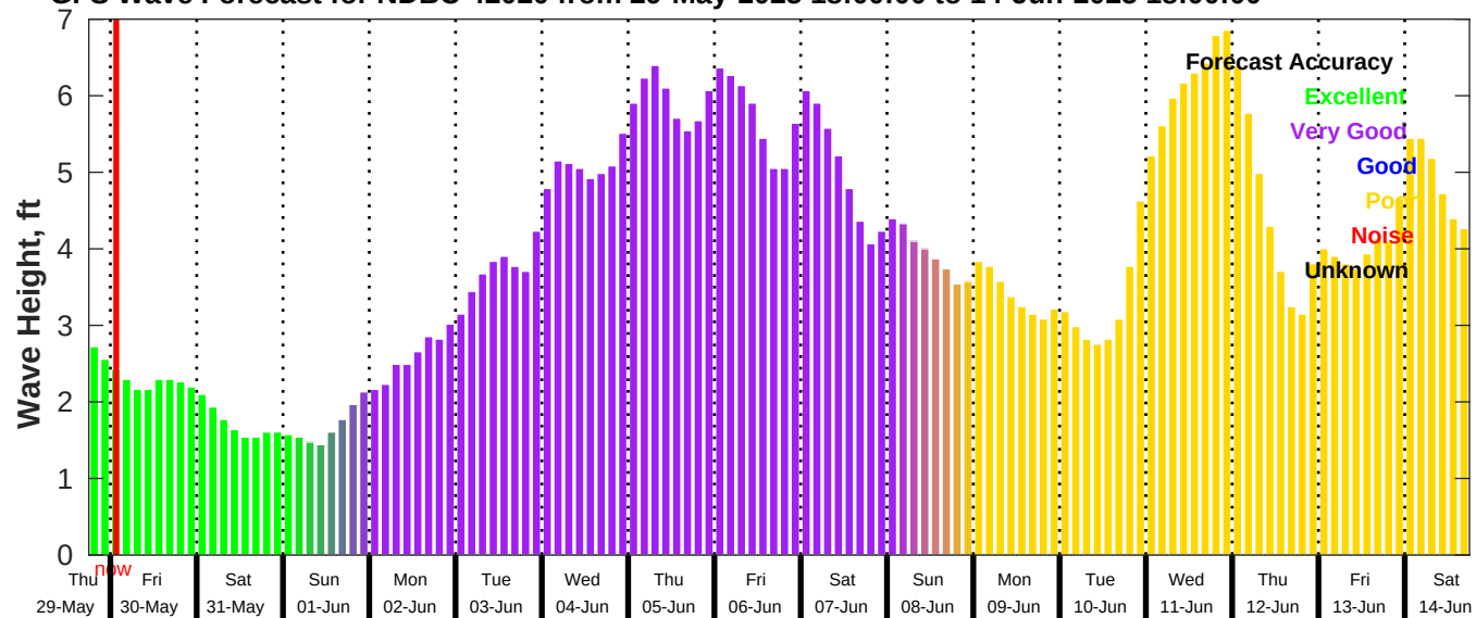
GFS Wave Forecast for NDBC 42020 from 29-May-2025 18:00:00 to 14-Jun-2025 18:00:00
