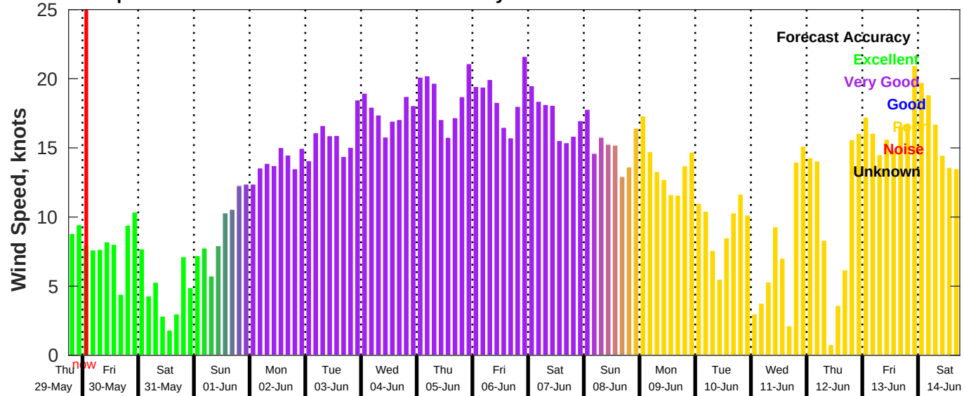
GFS Wind Speed Forecast for NDBC 42020 from 29-May-2025 18:00:00 to 14-Jun-2025 18:00:00
