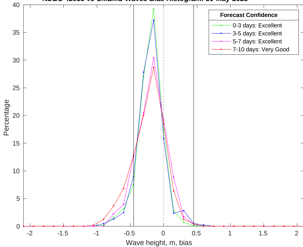
NDBC 42035 vs CMEMS Waves Bias Histogram: 30-May-2025
