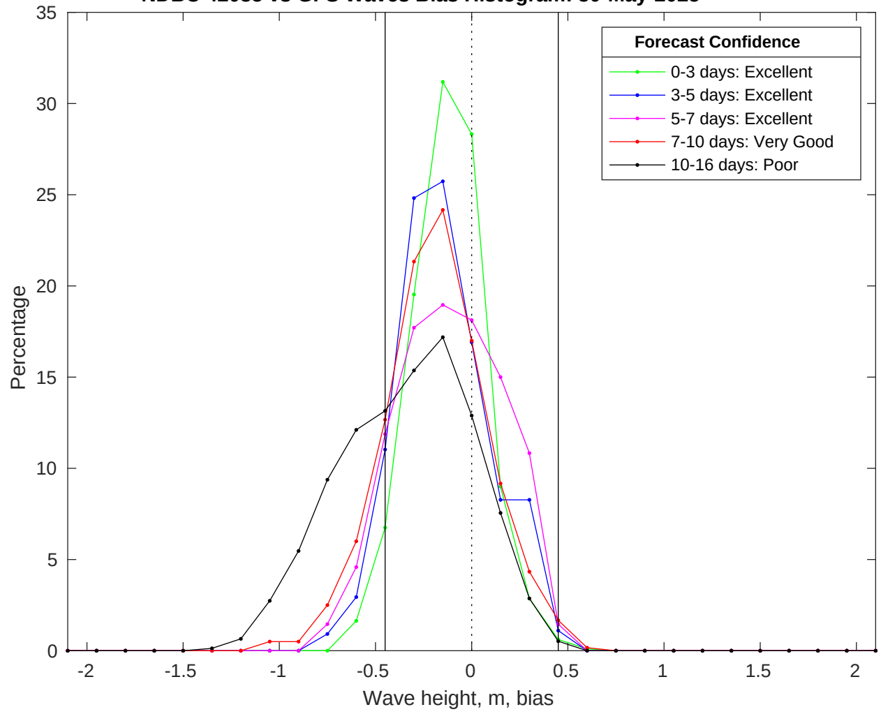
NDBC 42035 vs GFS Waves Bias Histogram: 30-May-2025
