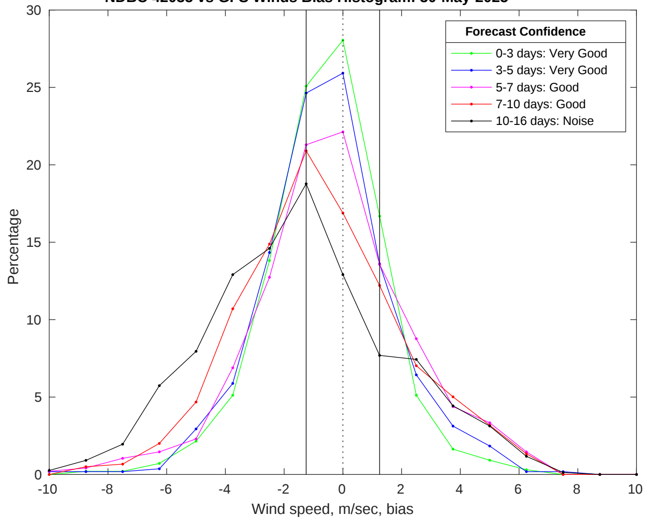
NDBC 42035 vs GFS Winds Bias Histogram: 30-May-2025
