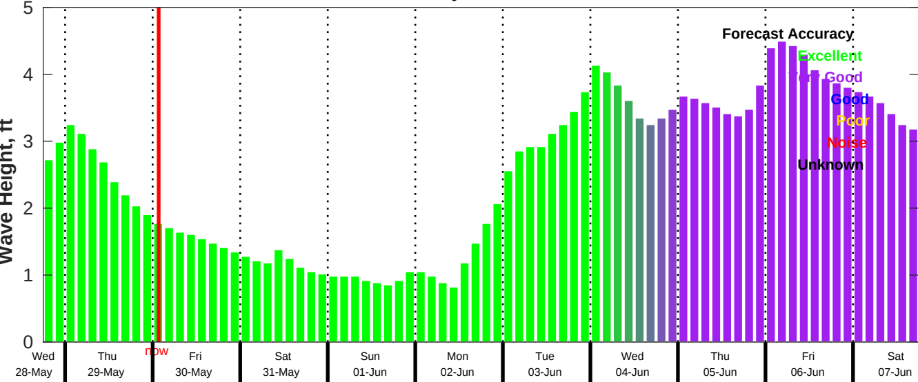
CMEMS Wave Forecast for NDBC 42035 from 28-May-2025 18:00:00 to 07-Jun-2025 18:00:00
