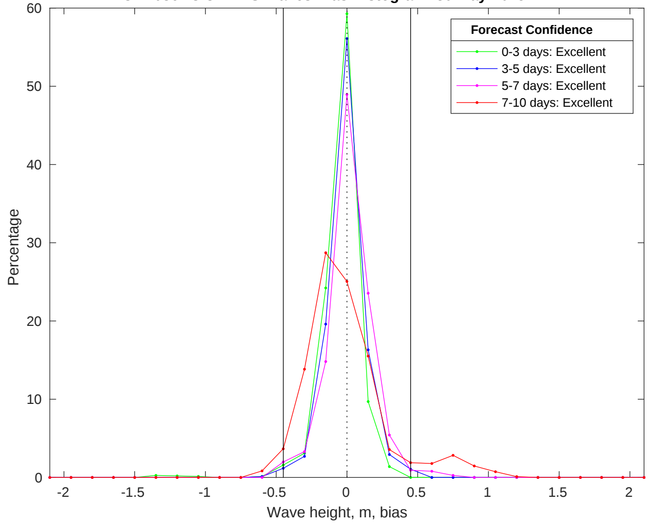
NDBC 42036 vs CMEMS Waves Bias Histogram: 30-May-2025
