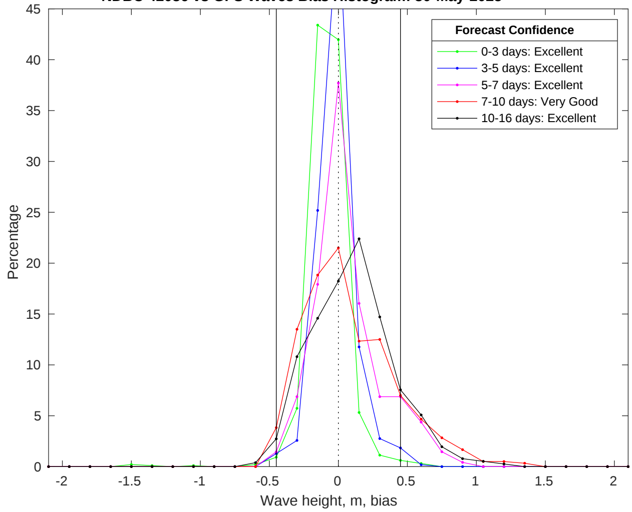
NDBC 42036 vs GFS Waves Bias Histogram: 30-May-2025
