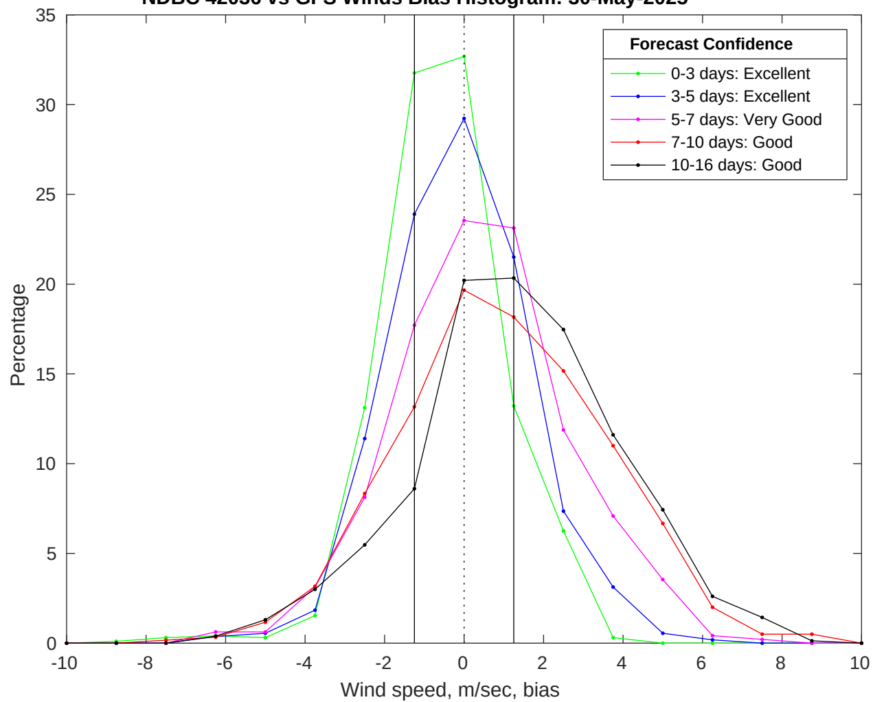
NDBC 42036 vs GFS Winds Bias Histogram: 30-May-2025
