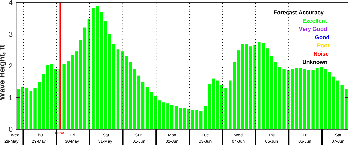
CMEMS Wave Forecast for NDBC 42036 from 28-May-2025 19:00:00 to 07-Jun-2025 19:00:00
