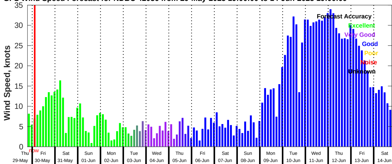
GFS Wind Speed Forecast for NDBC 42036 from 29-May-2025 19:00:00 to 14-Jun-2025 19:00:00
