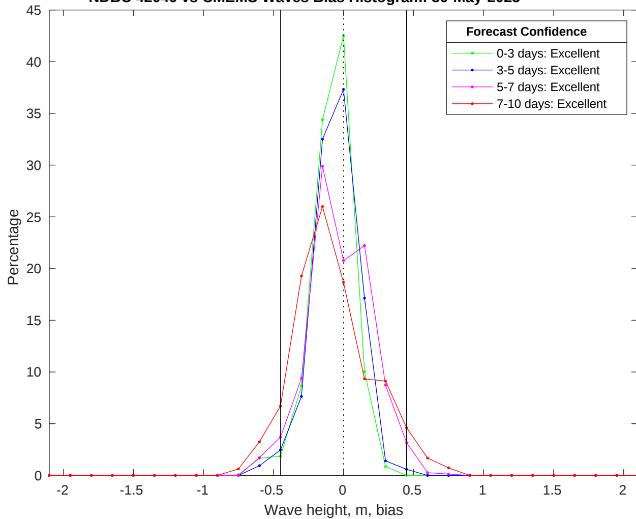
NDBC 42040 vs CMEMS Waves Bias Histogram: 30-May-2025
